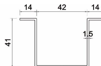
Code: PDA1922 L : 6.0m G AL : 1.64kg/m
