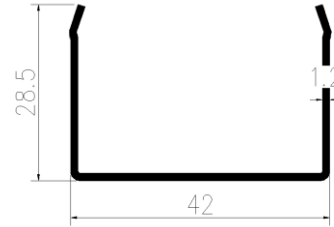
Code: PDA1923CA L : 6.0m G : 0.91kg/m
